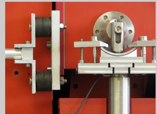
False Brinelling
